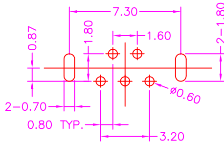
P.C.B LAYOUT TOP VIEW ±0.05
