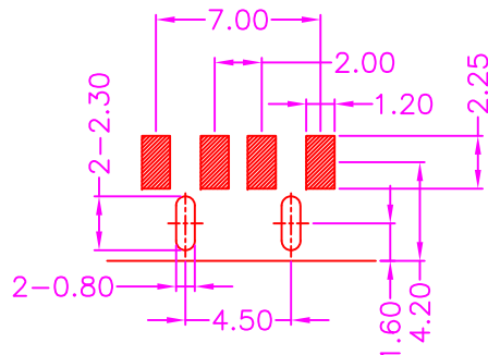
P.C.B. LAYOUT TOP VIEW ±0.05
