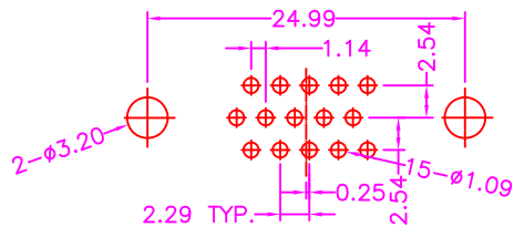
P.C.B LAYOUT TOP VIEW ±0.05
