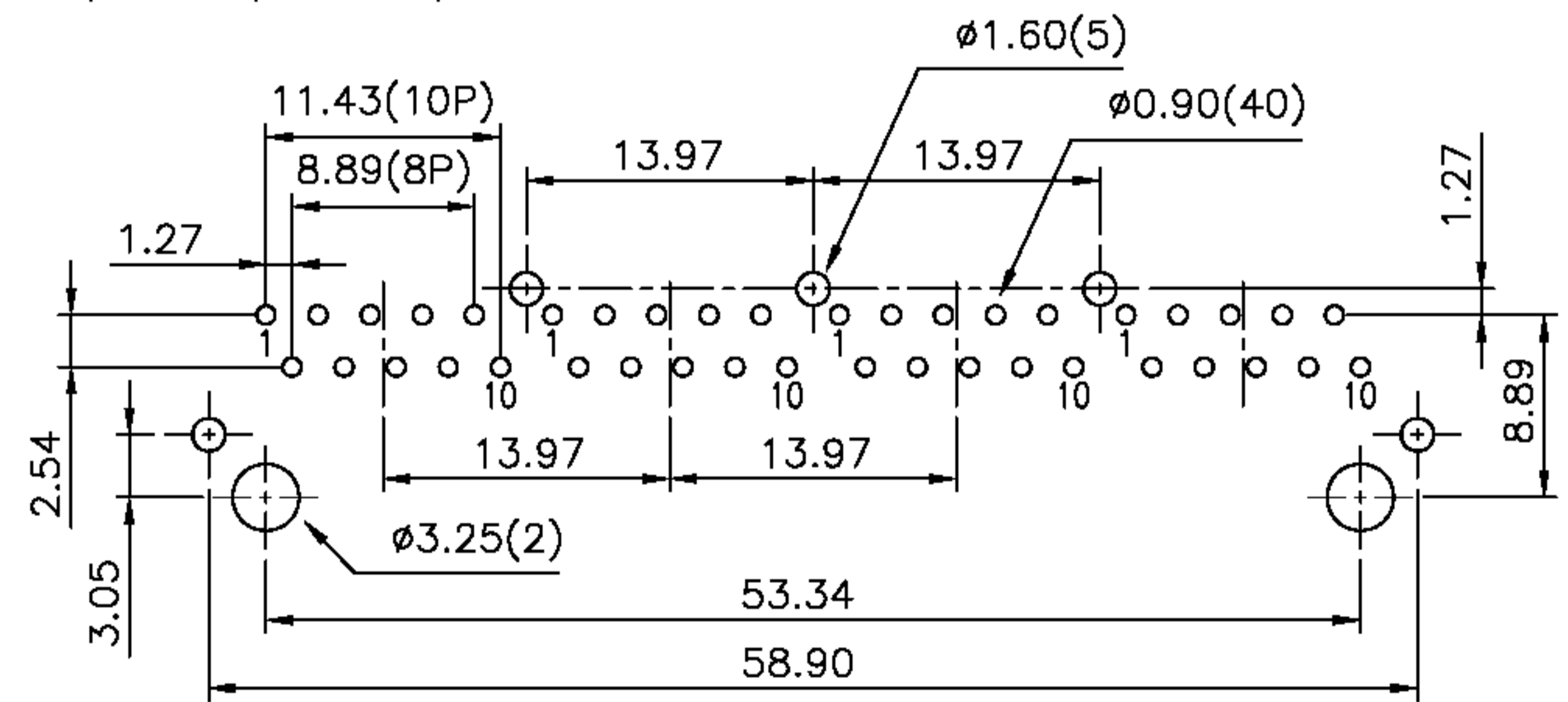
PCB LAYOUT Ref.
