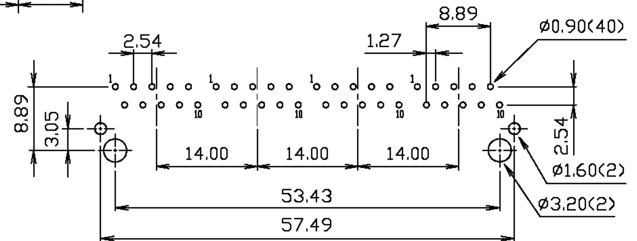
PCB LAYOUT
