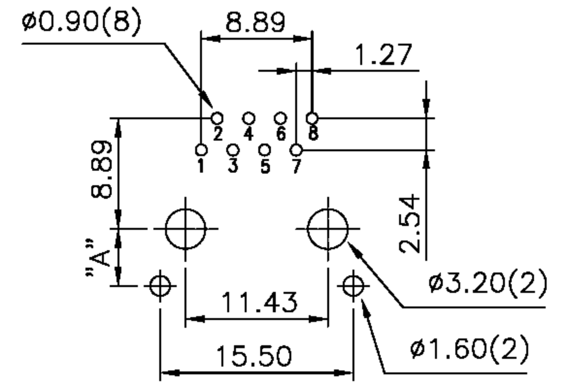
PCB LAYOUT Ref.
