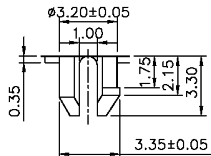
DETAIL X
