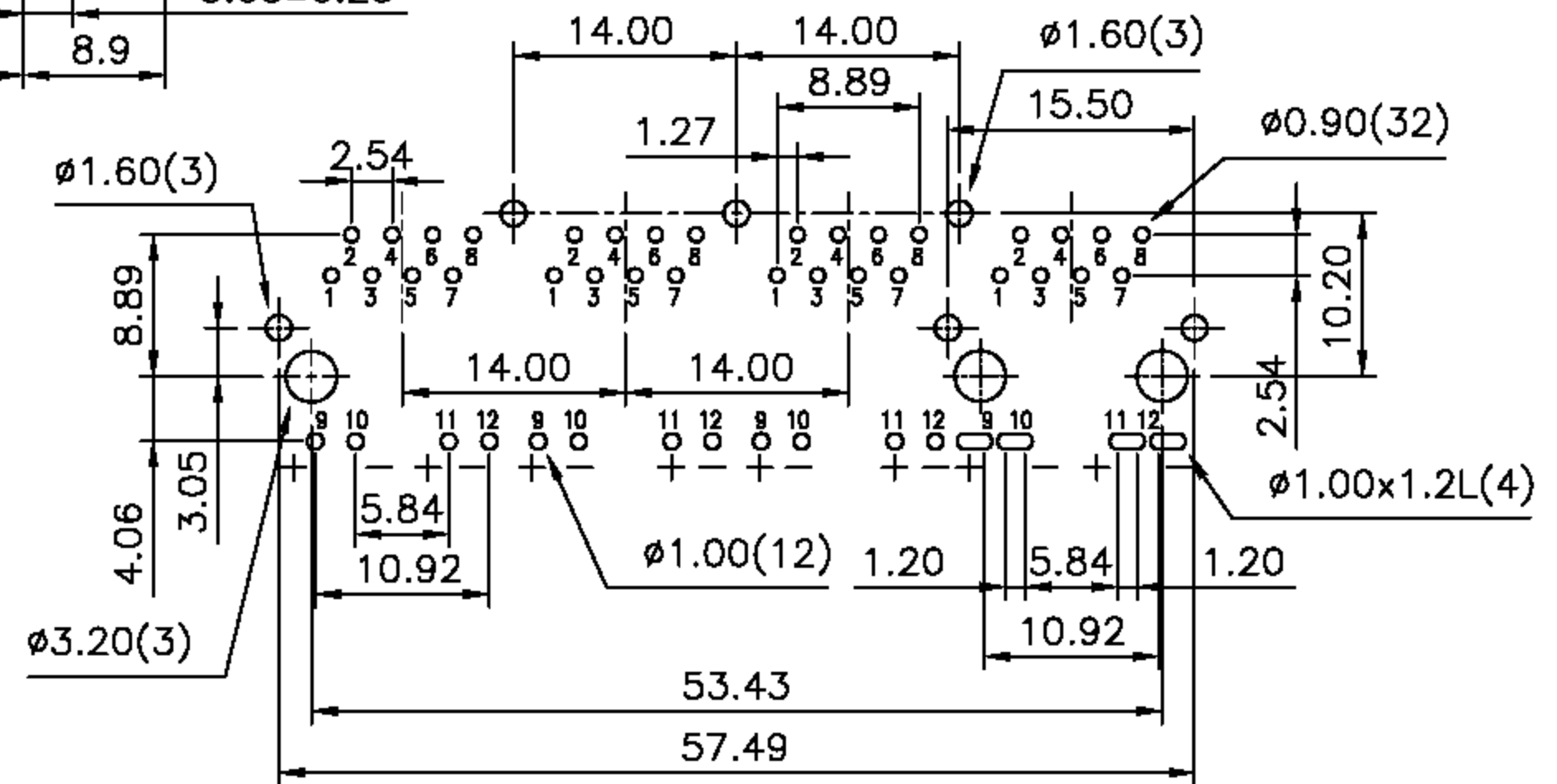
PCB LAYOUT
