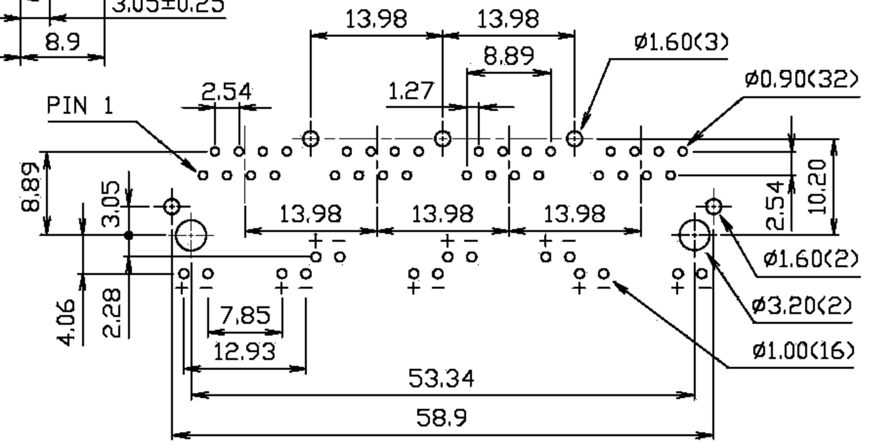
PCB LAYOUT
