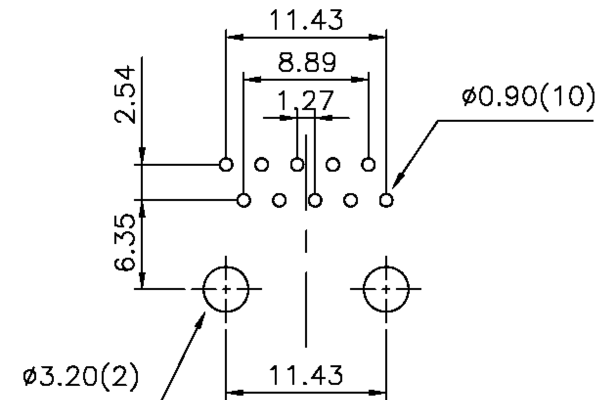
PCB LAYOUT
