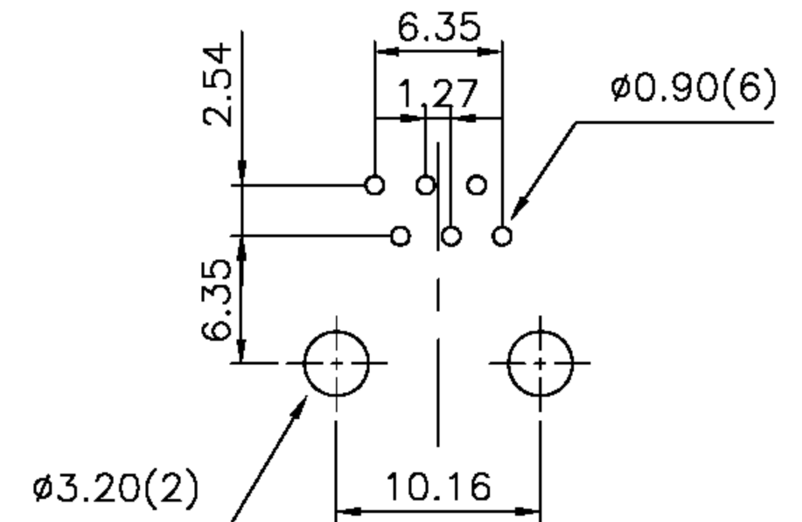
PCB LAYOUT
