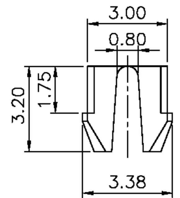
DETAIL X
