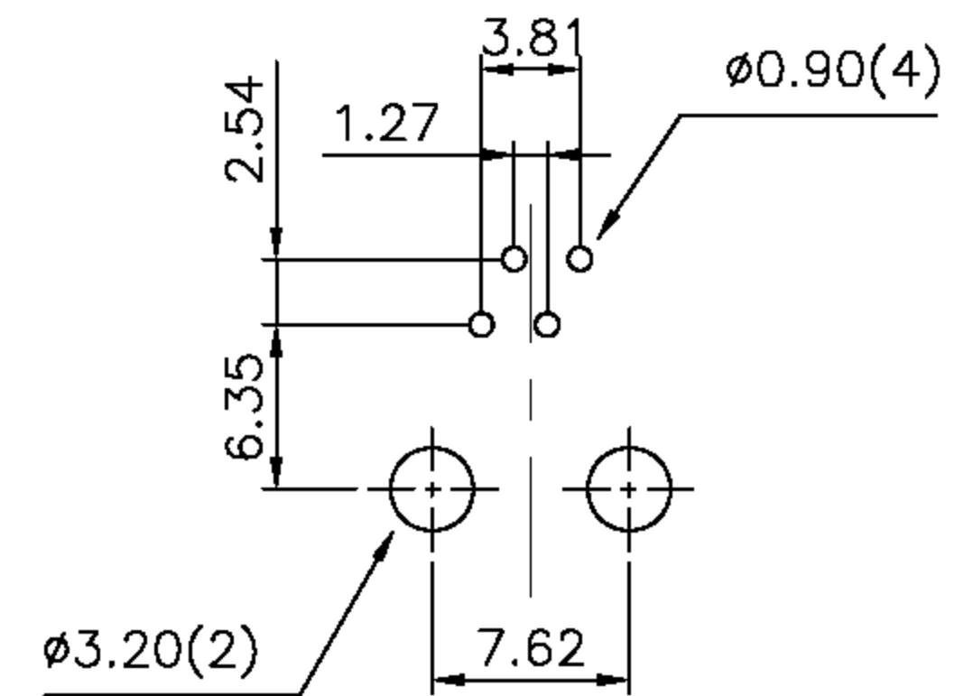
PCB LAYOUT
