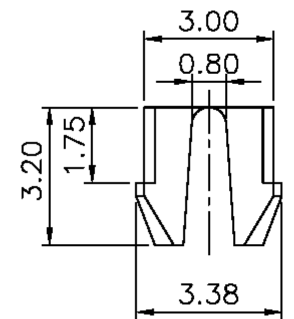
DETAIL X
