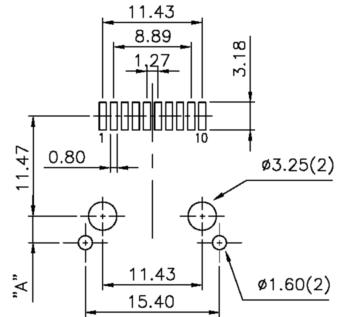
PCB LAYOUT
