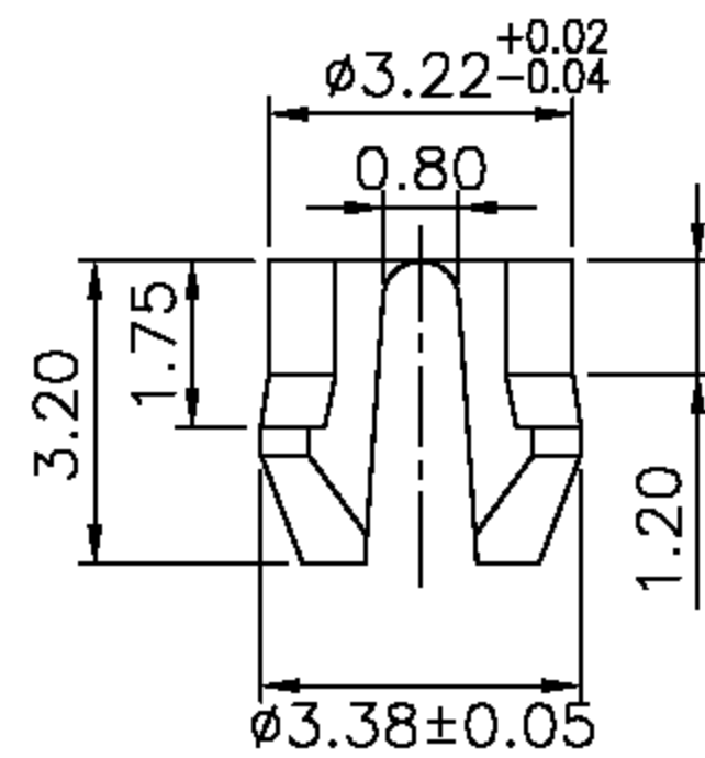
DETAIL X
