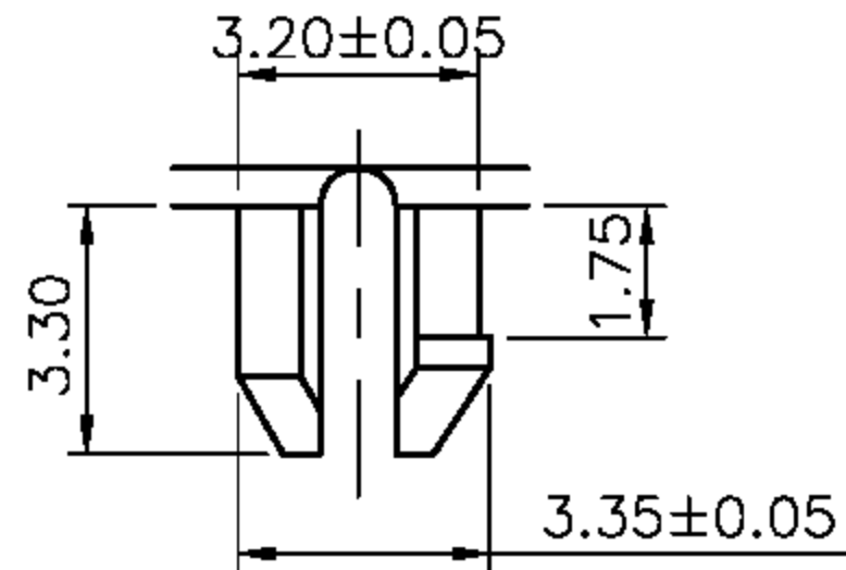
DETAIL X
