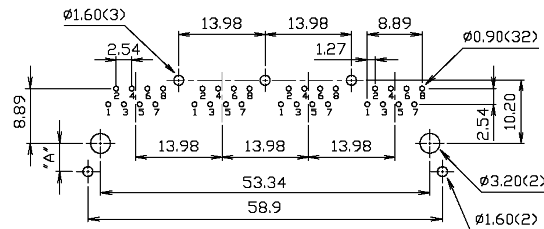
PCB LAYOUT Ref.
