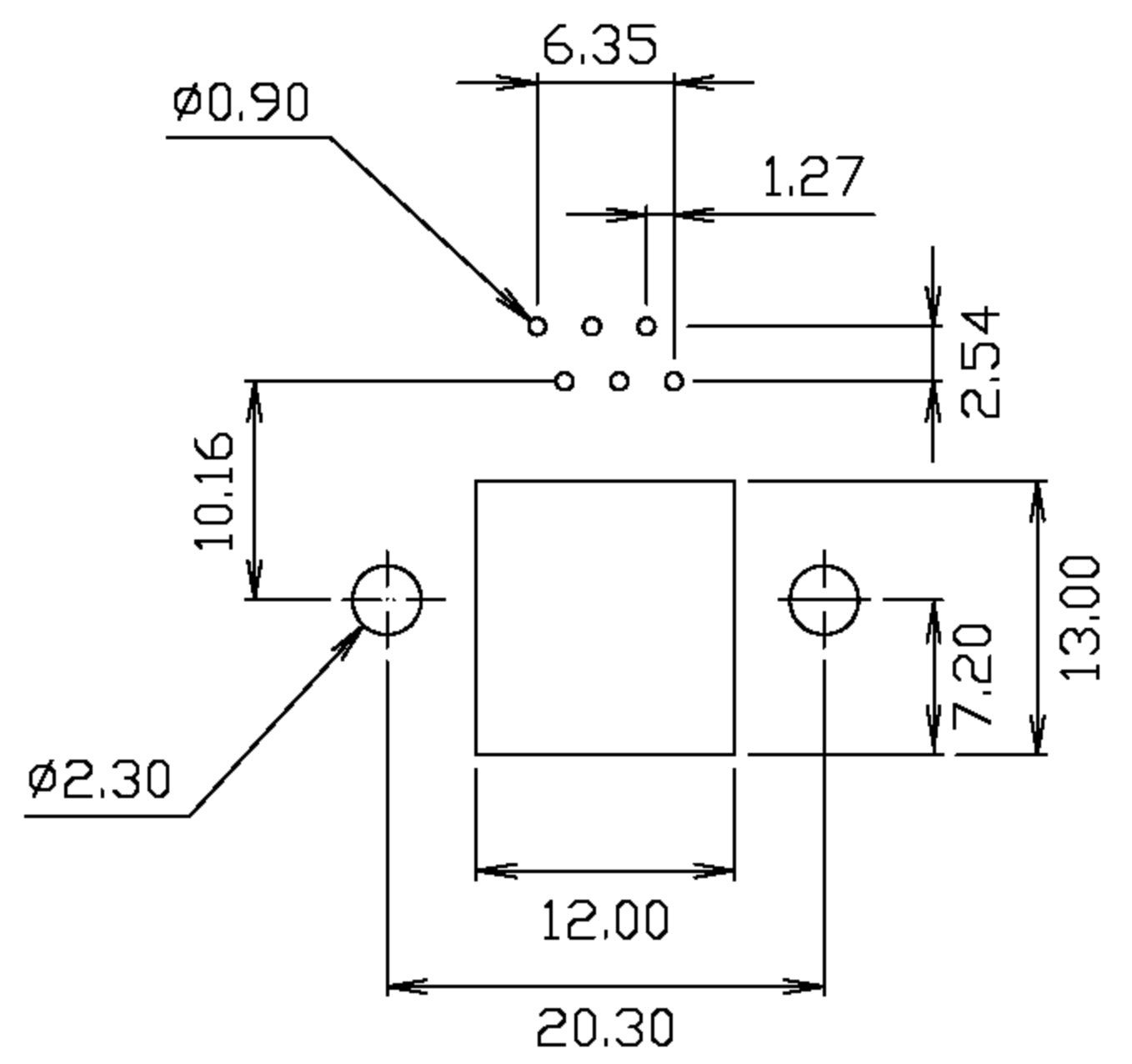
PC Board Layout
