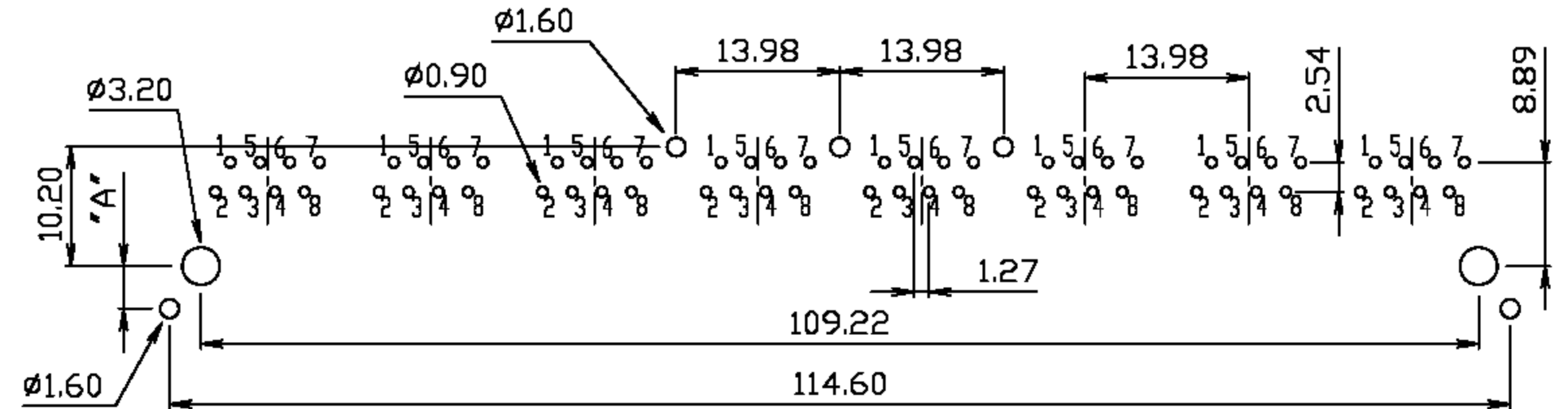
PC Board Layout REF.
