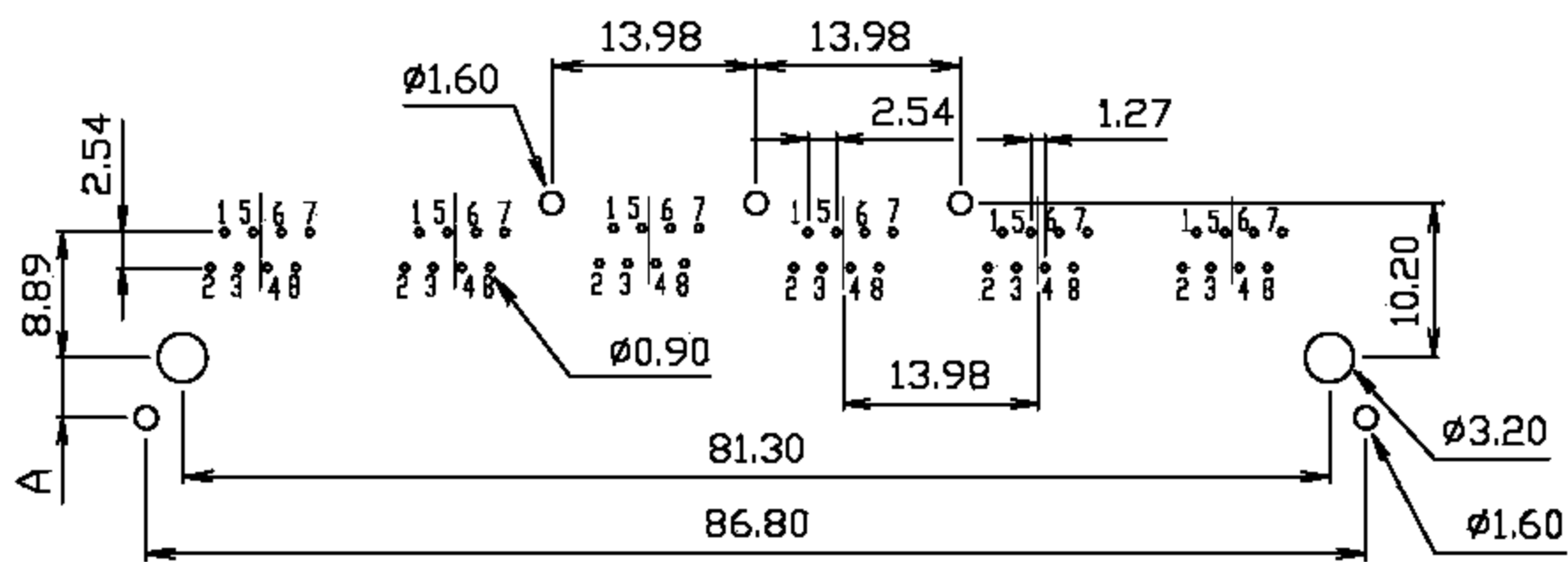
6PORTS PC Board Layout
