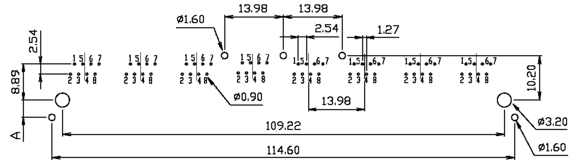
8PORTS PC Board Layout
