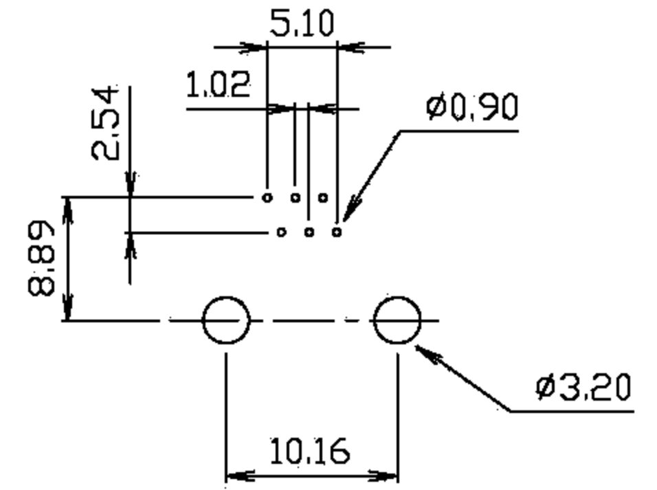
PC Board Layout
