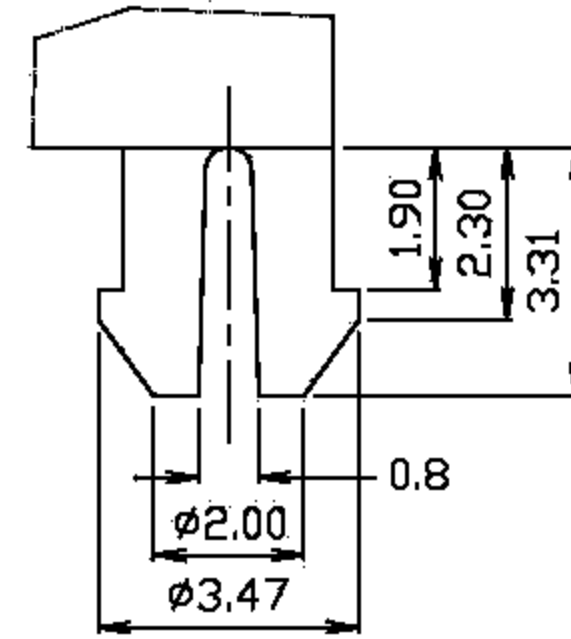
DETAIL X
