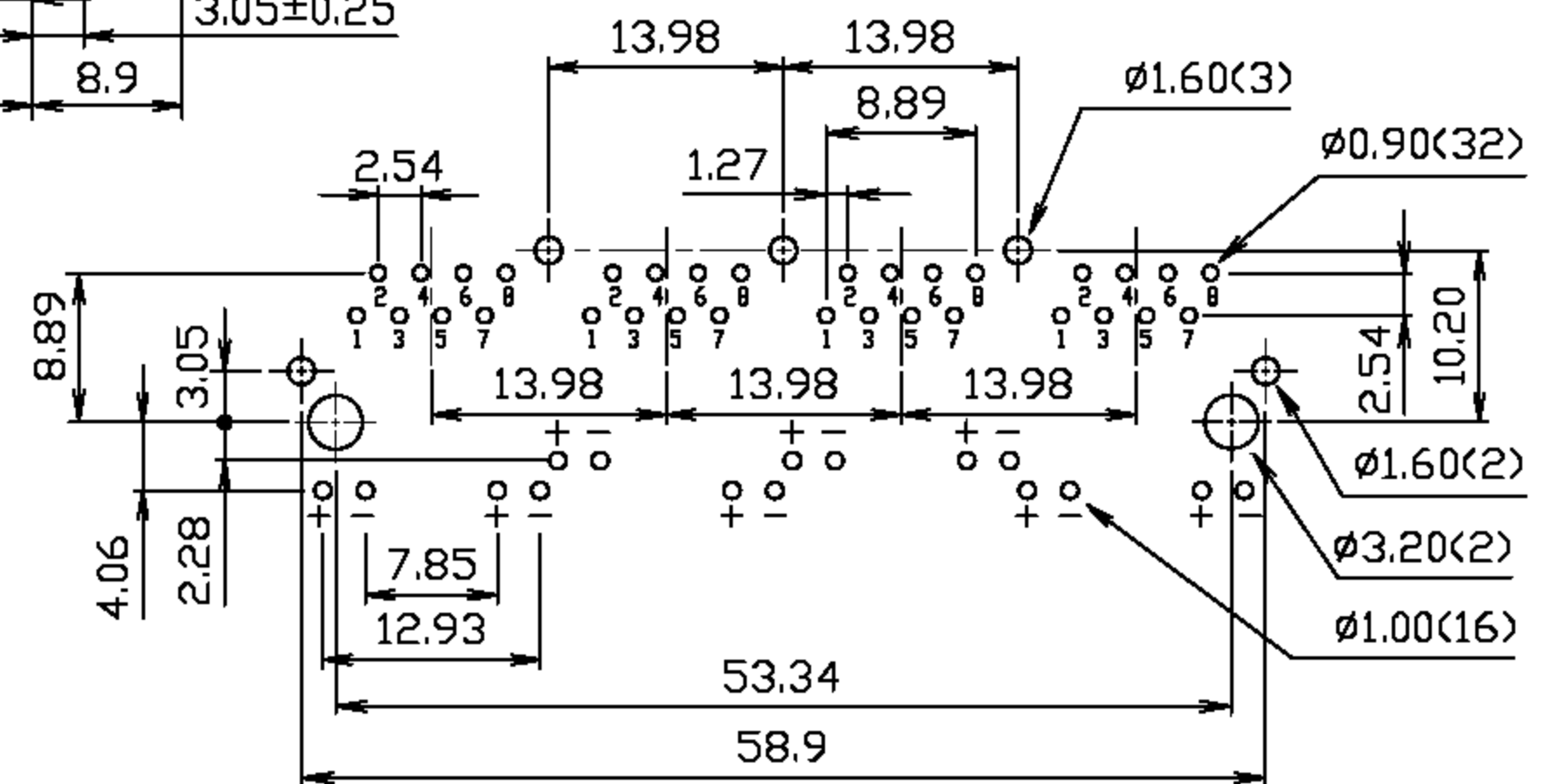
PCB LAYOUT
