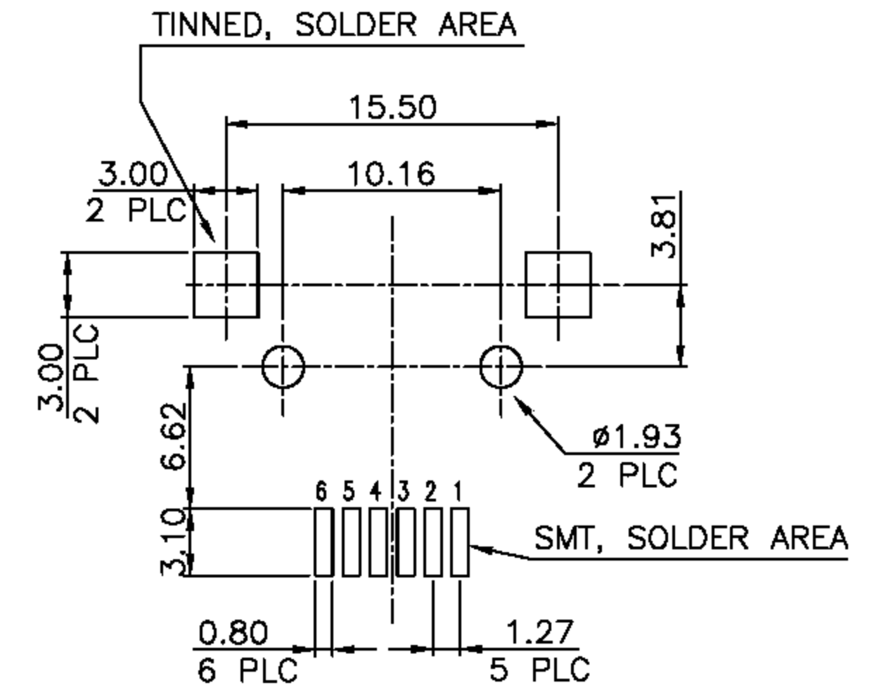
PCB LAYOUT
