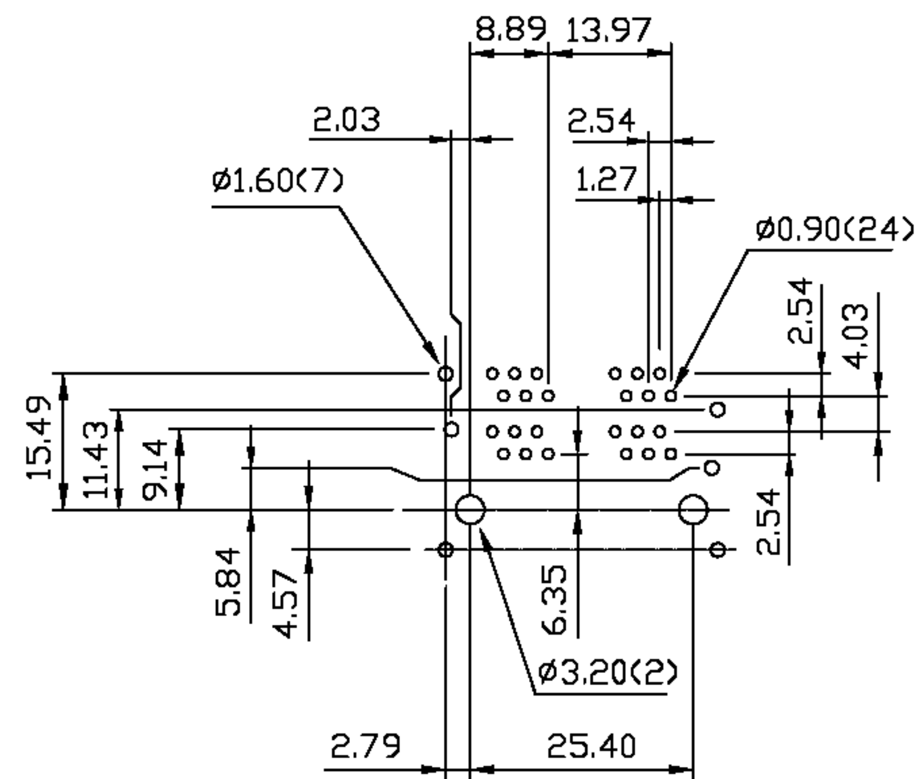
PCB LAYOUT
