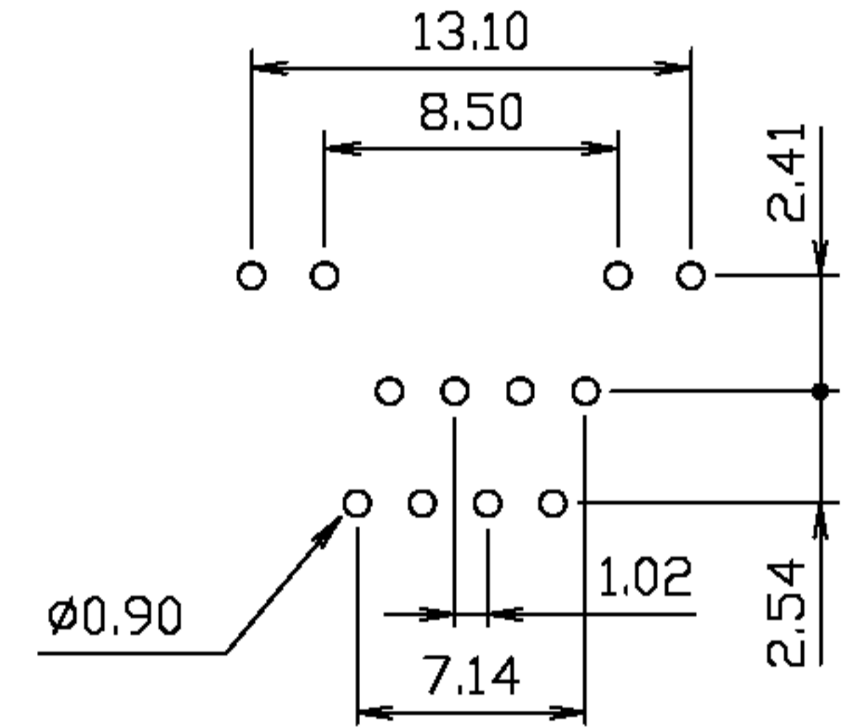
PCB LAYOUT
