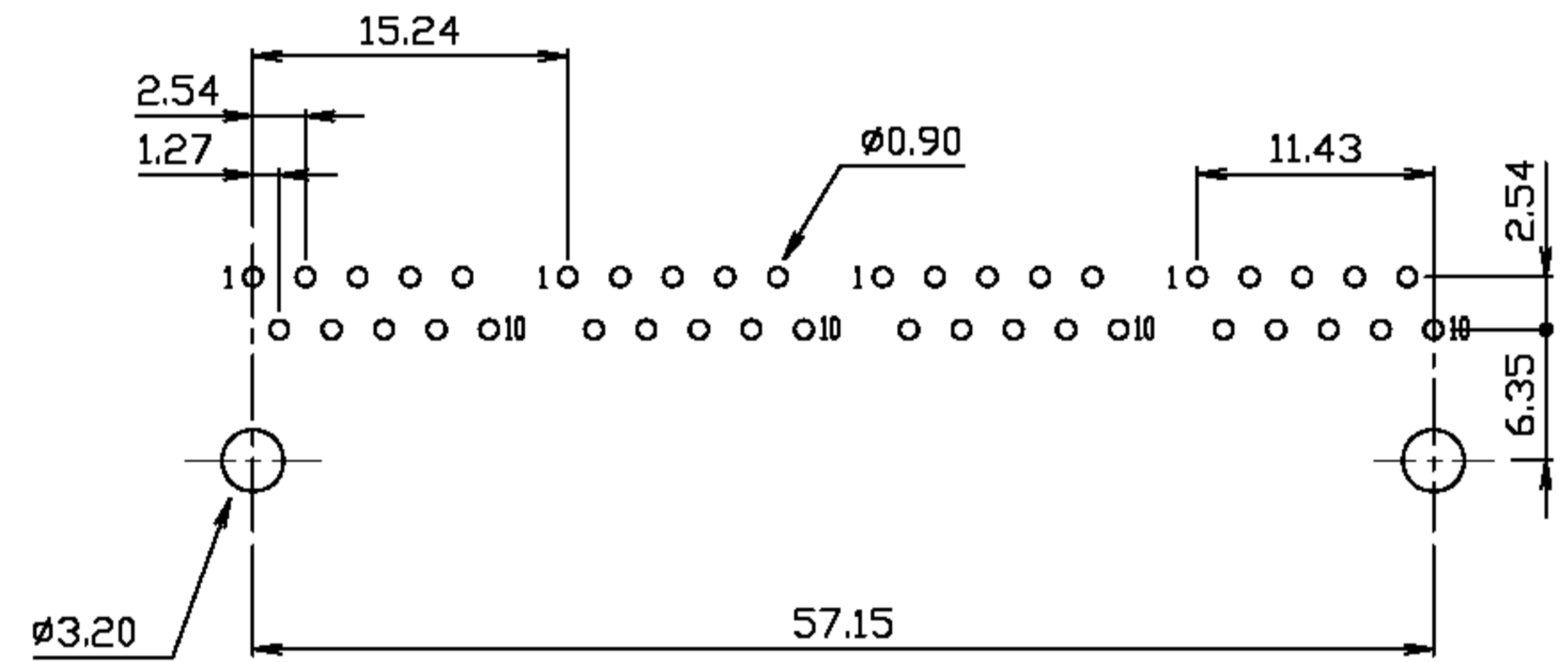
PC Board Layout Ref.
