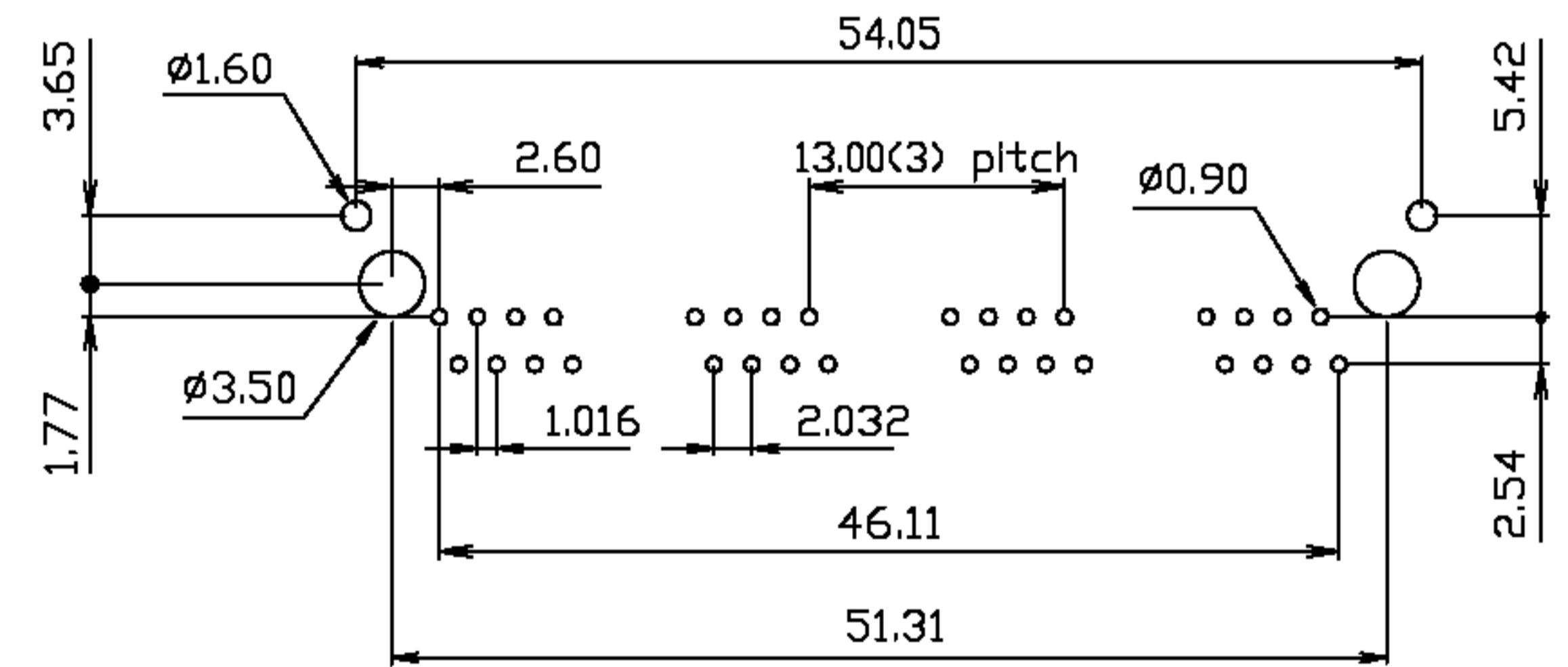
PCB LAYOUT
