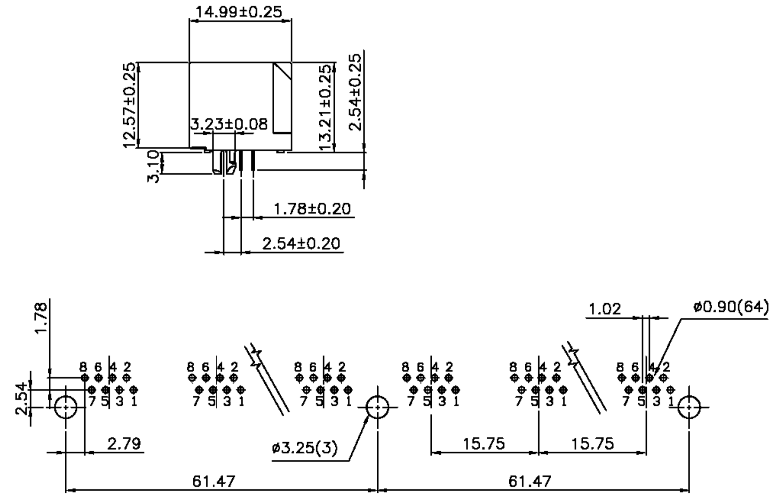
PCB Layout (Ref.)
