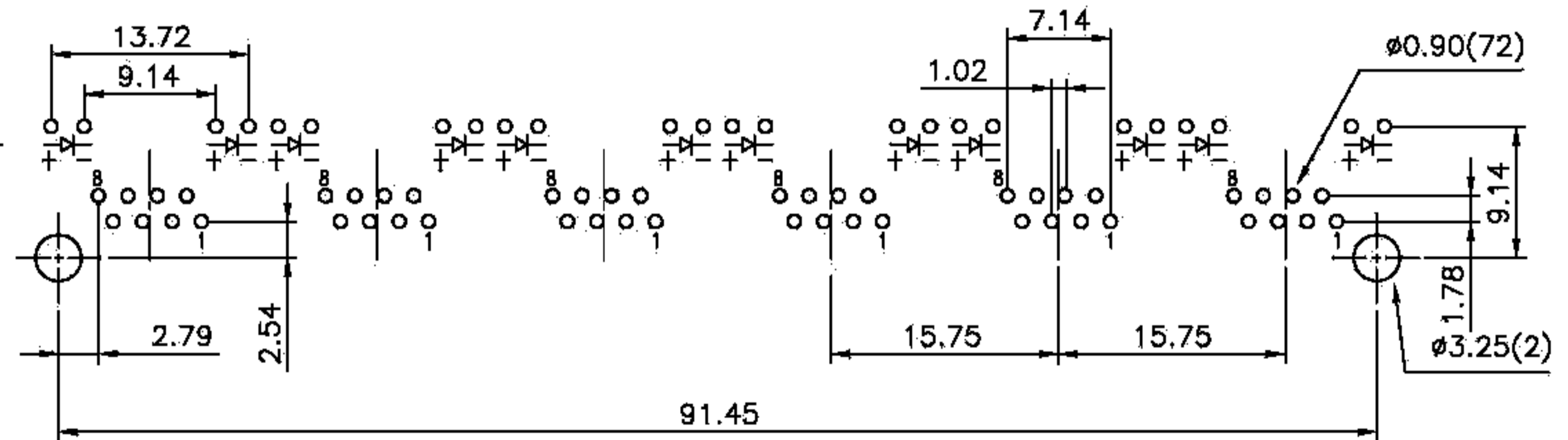
PCB Layout (Ref.)
