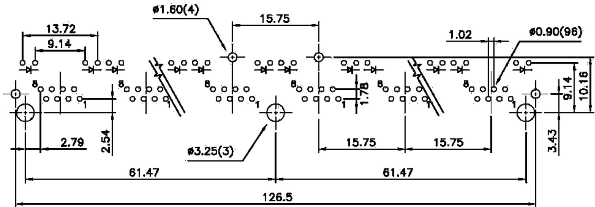
PCB Layout (Ref.)
