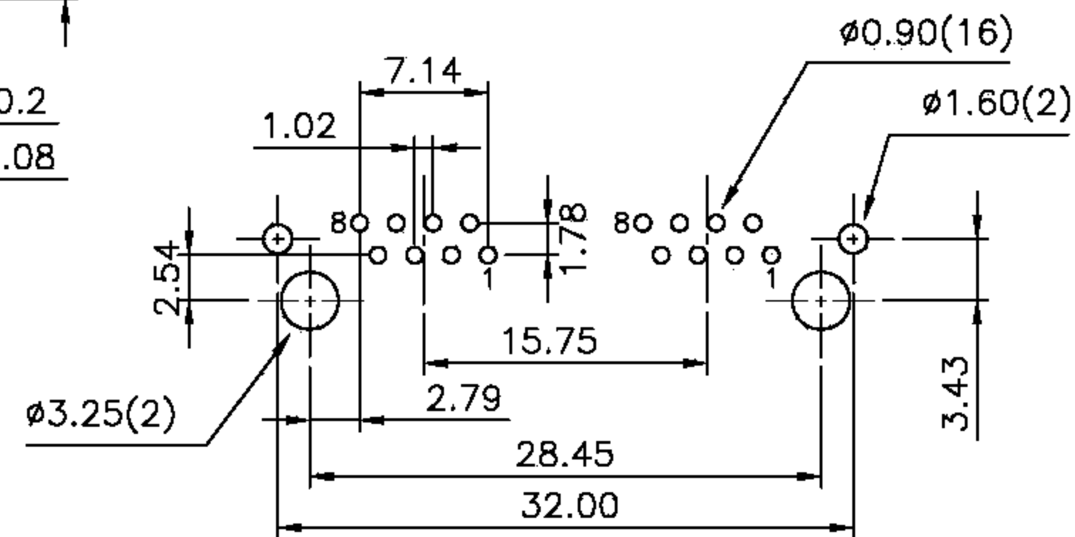
PCB LAYOUT (Ref.)
