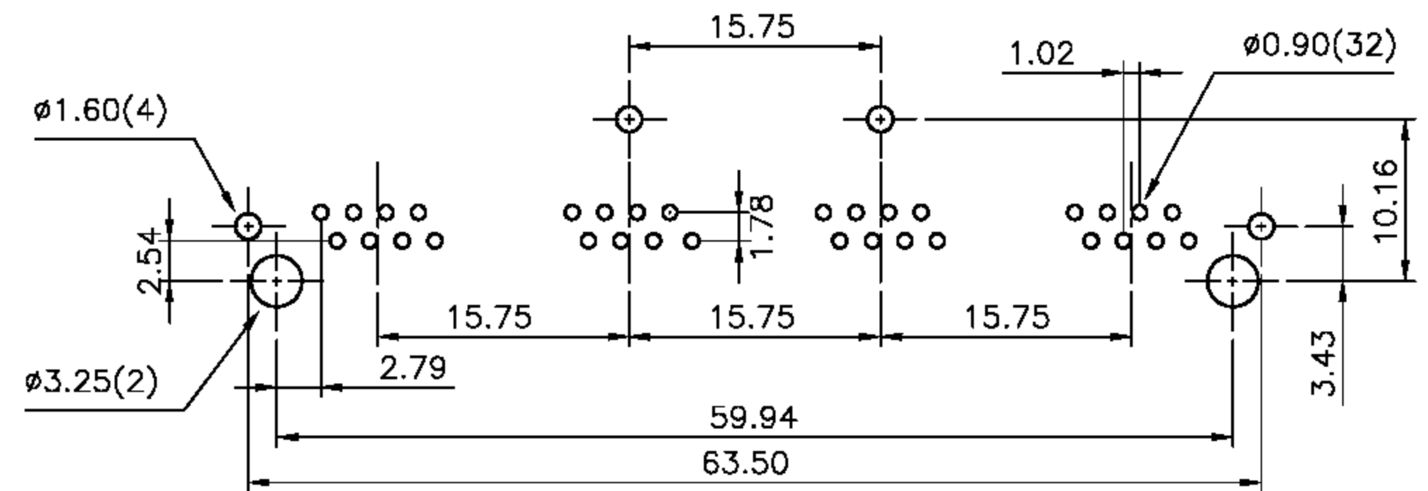
PCB LAYOUT (Ref.)
