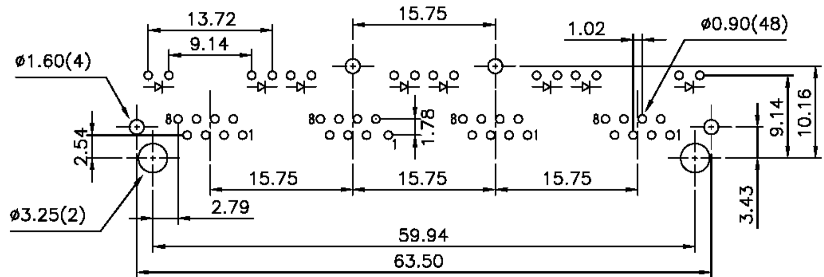
PCB LAYOUT (Ref.)
