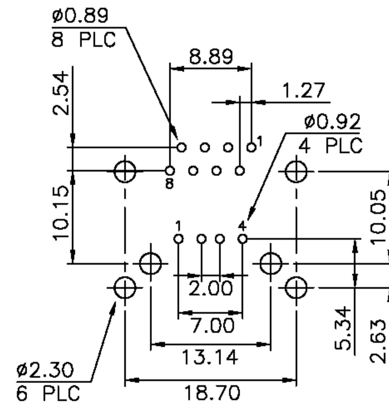
PCB LAYOUT Ref.
