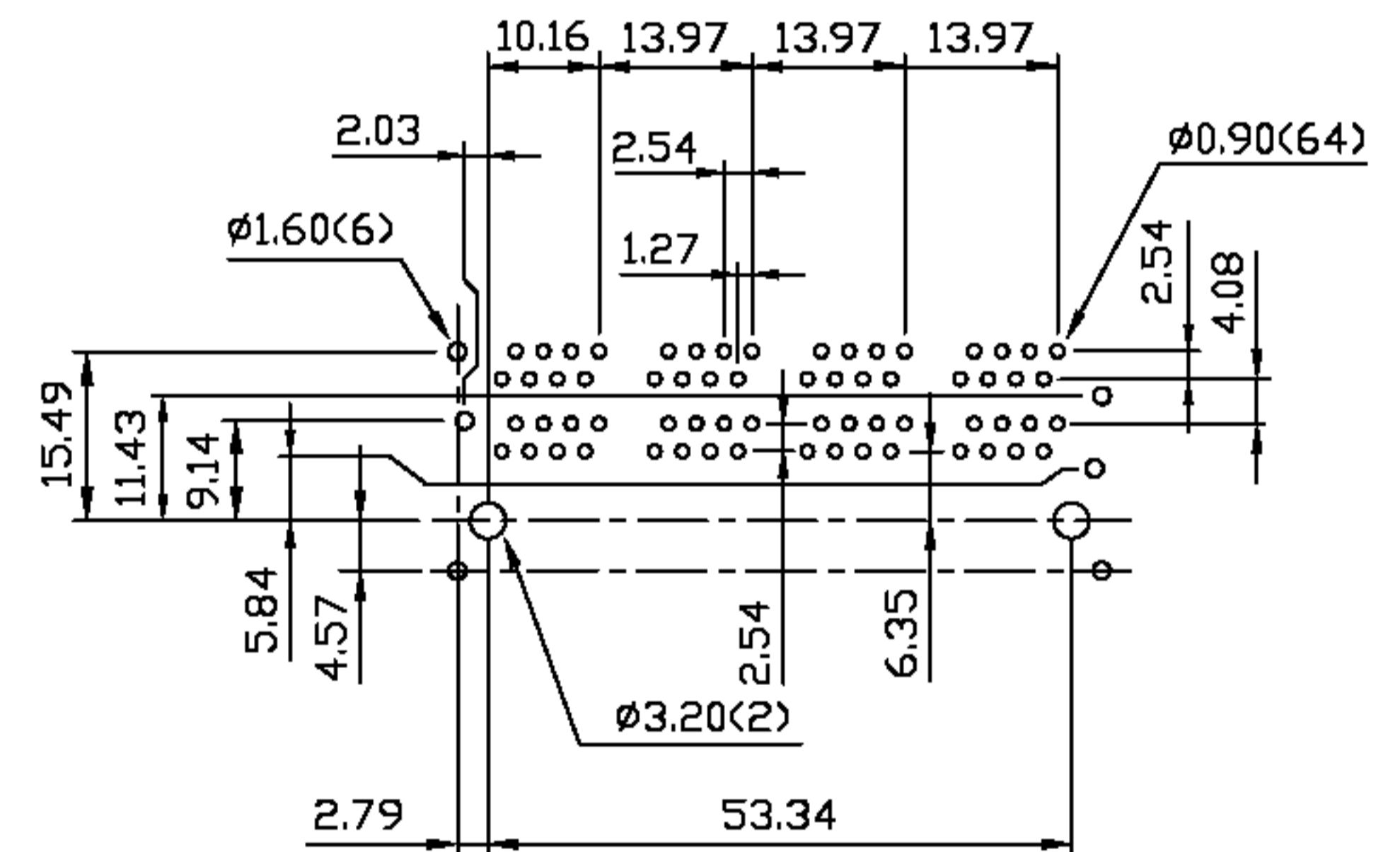
PCB LAYOUT
