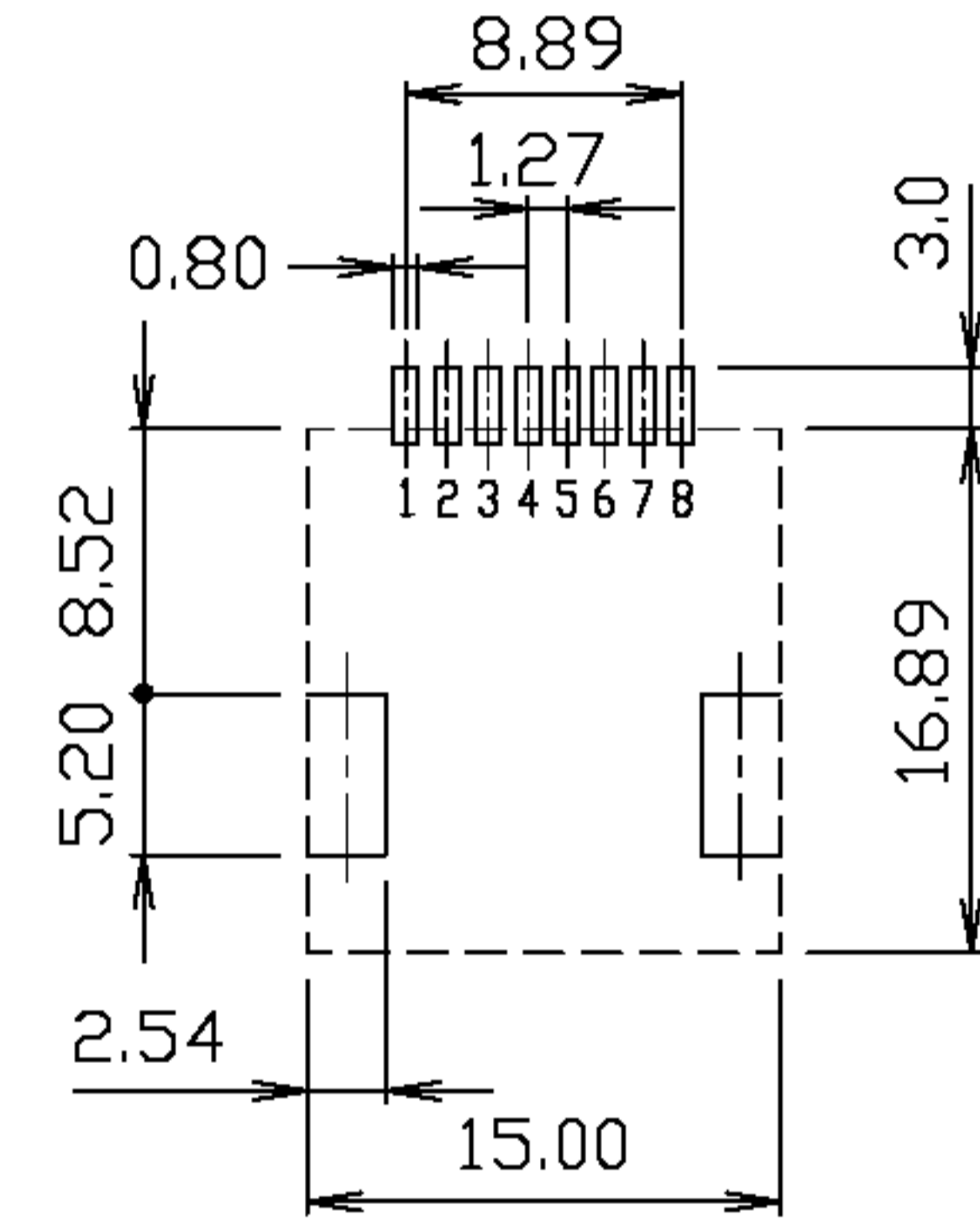
PCB LAYOUT Ref.
