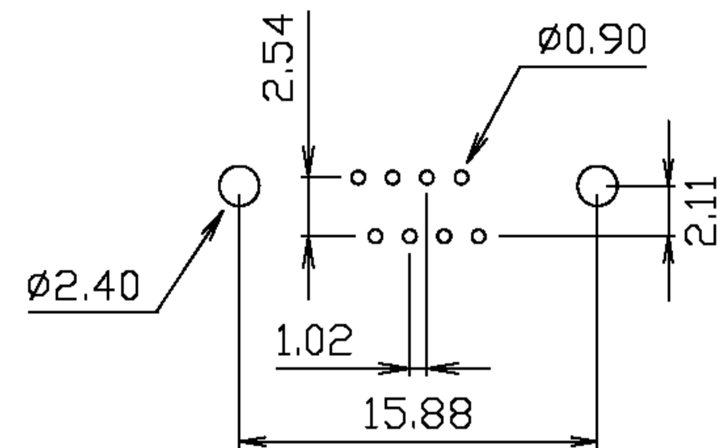
PC Board Layout
