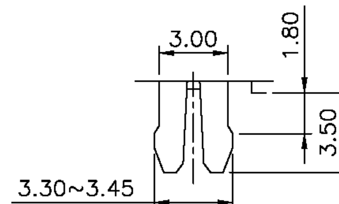
DETAIL X
