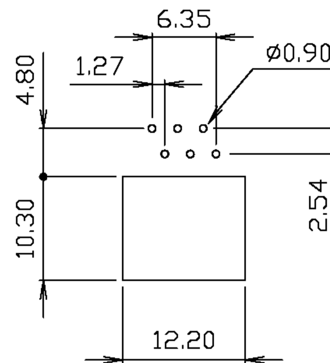
PC Board Layout
