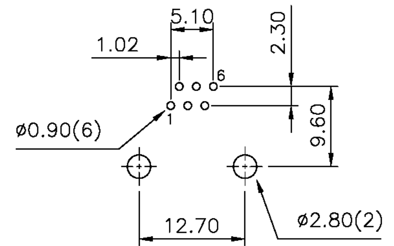
PC Board Layout Ref.
