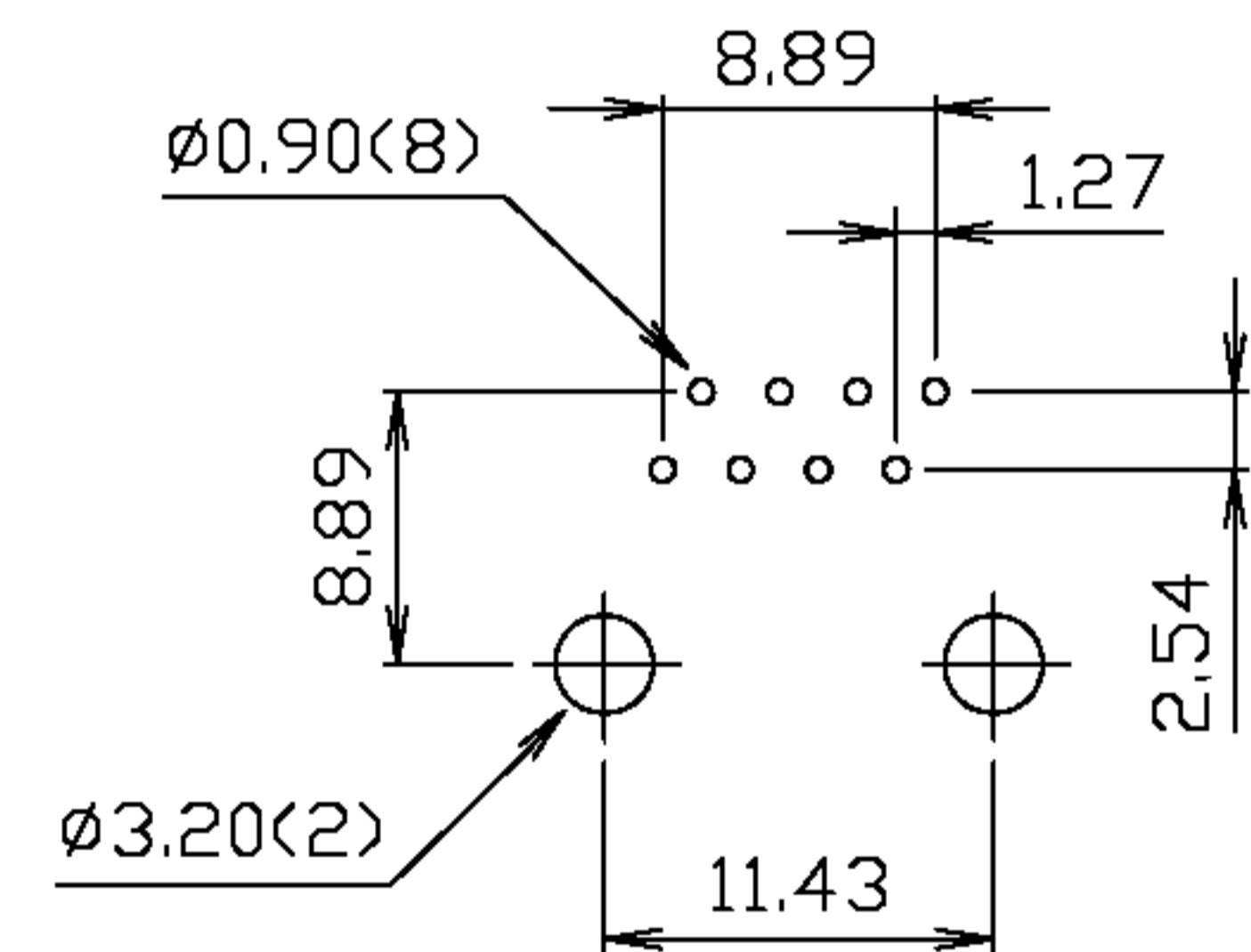
PC Board Layout
