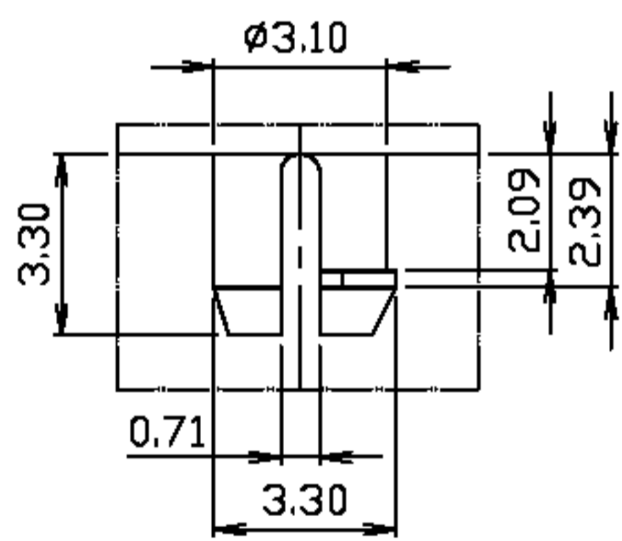
DETAIL X
