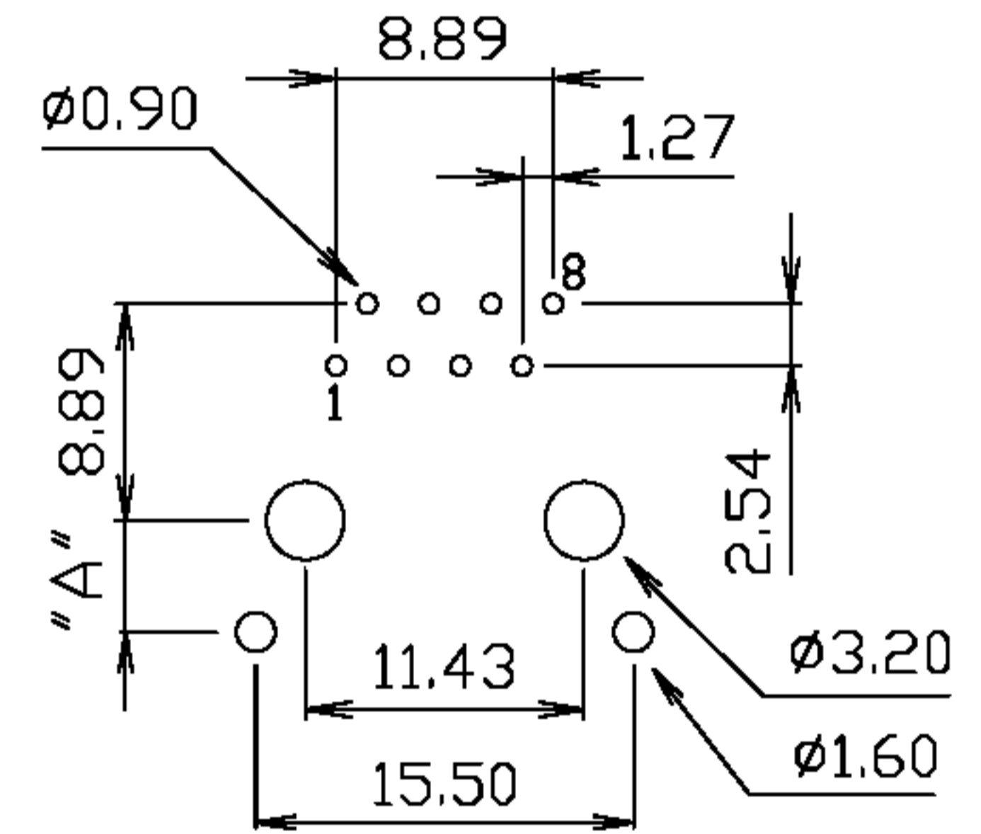
PCB LAYOUT Ref.
