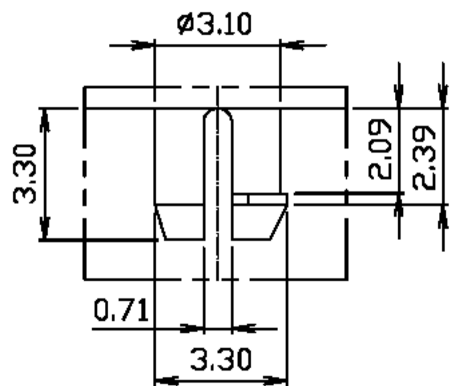
DETAIL X
