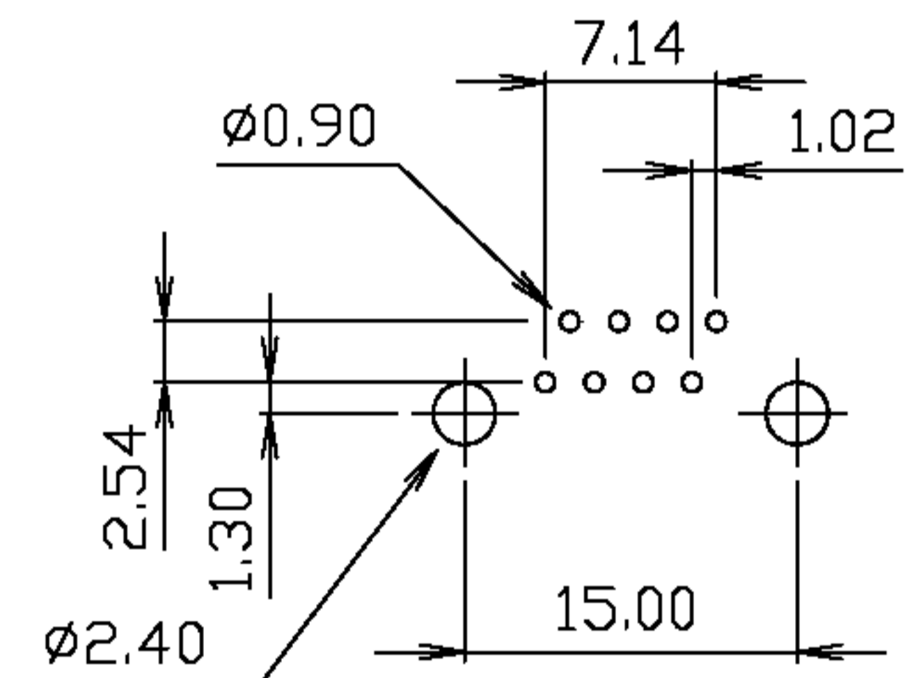
PC Board Layout
