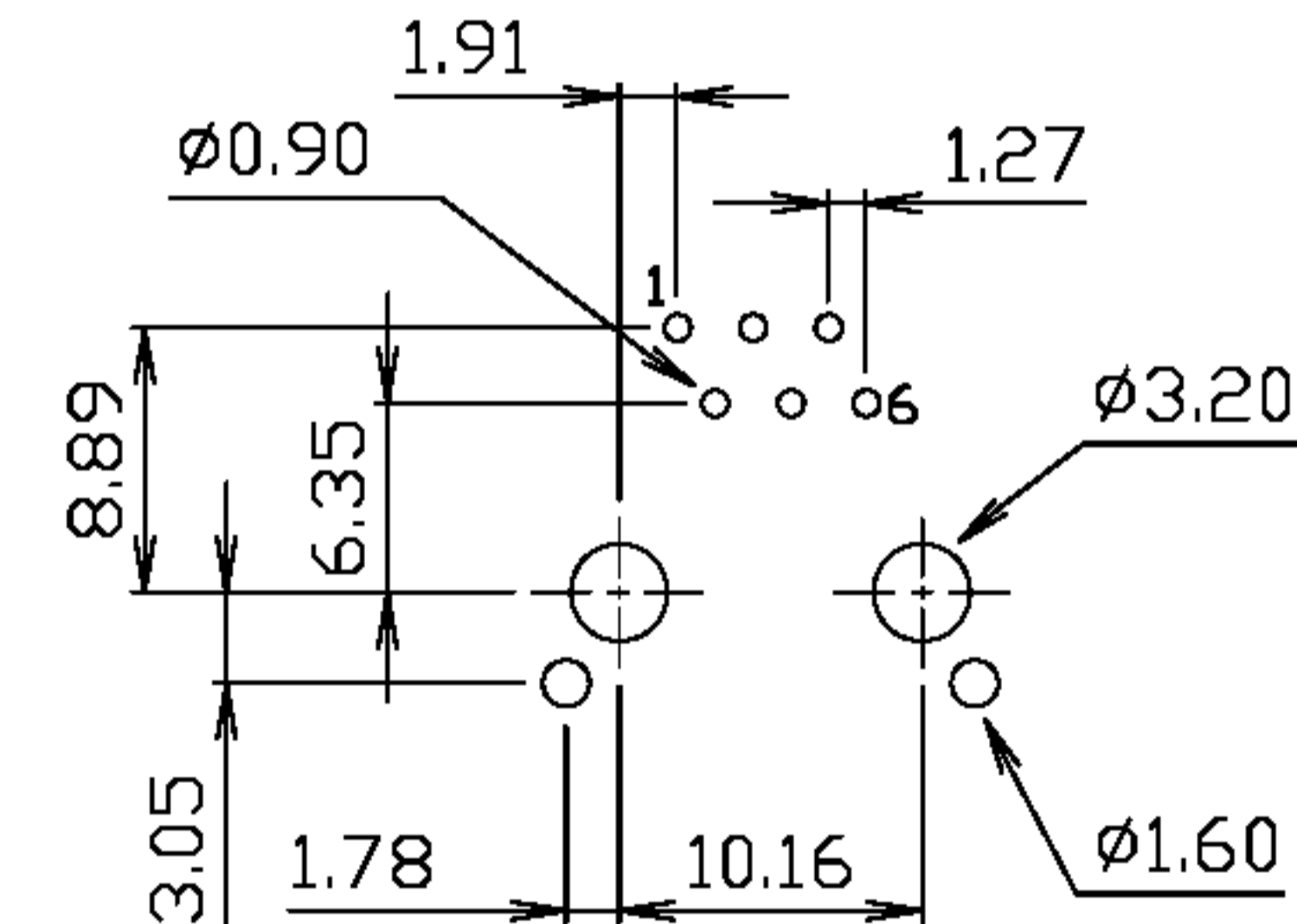
PC Board Layout Ref.
