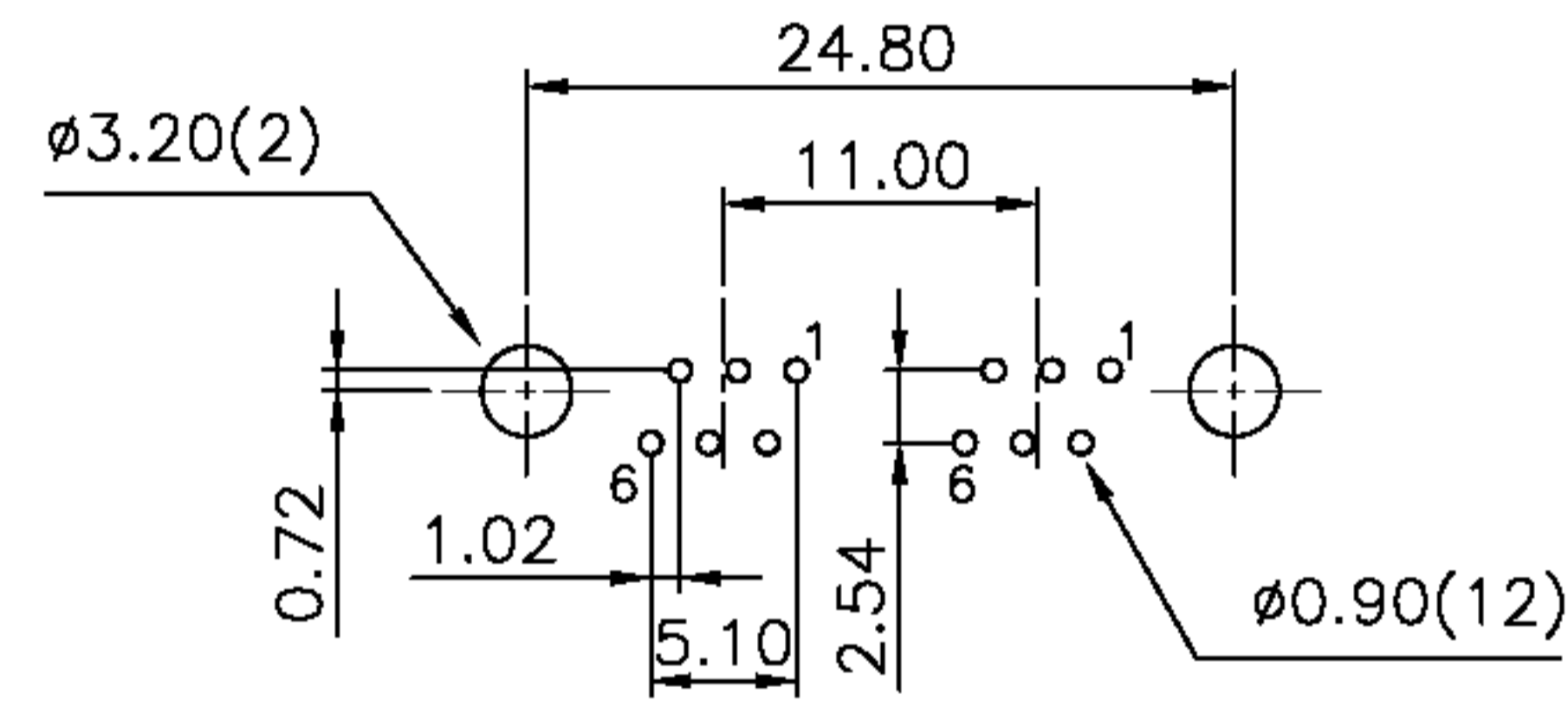
PC Board Layout Ref.
