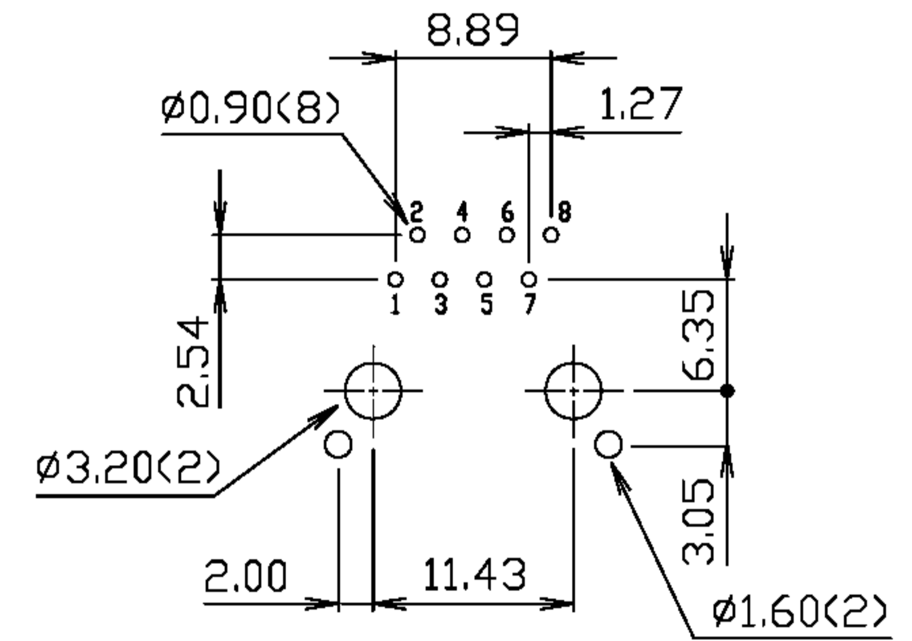
PC Board Layout Ref.
