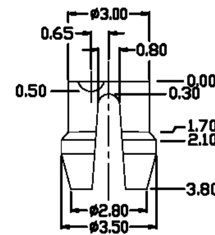
DETAIL X
