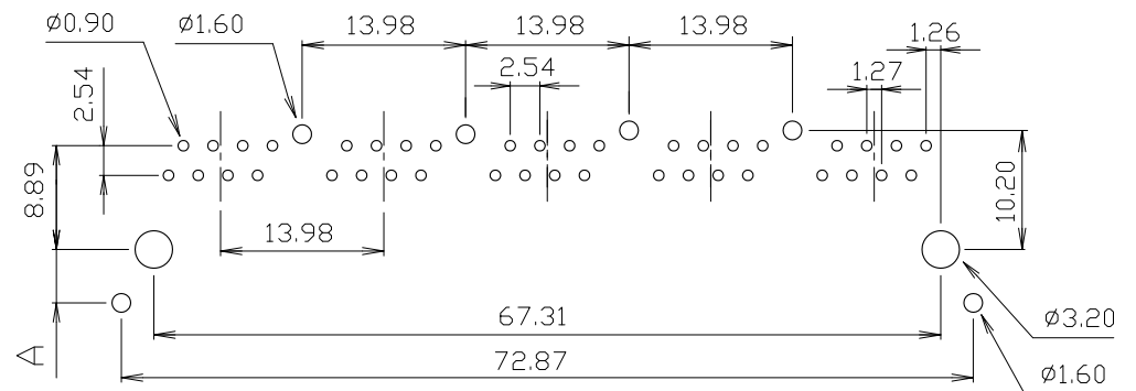
PC Board Layout Ref.
