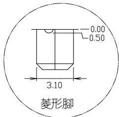
DIAMOND PEGS
