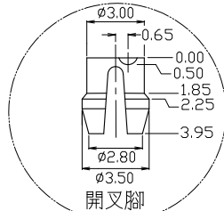
SPLIT-PEGS
