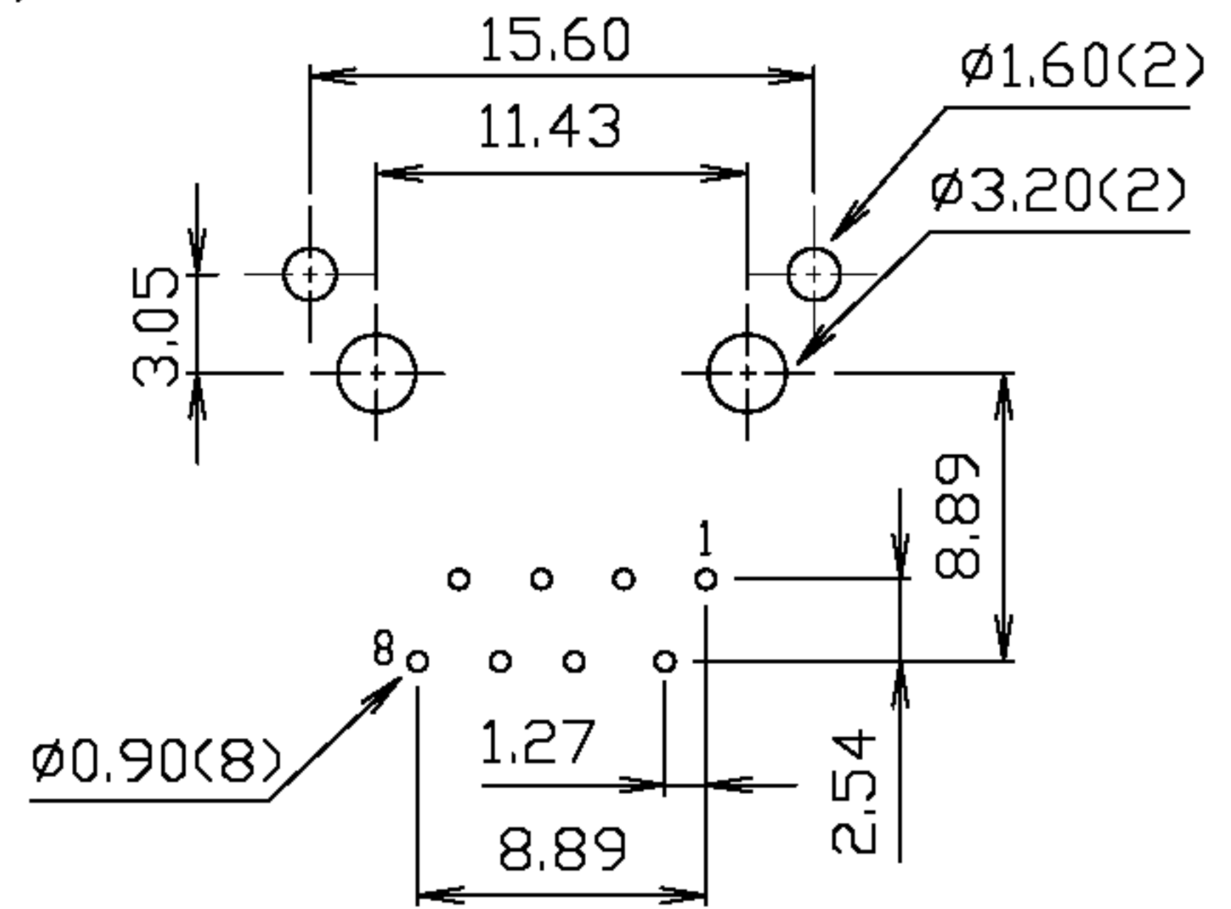
PC Board Layout Ref.
