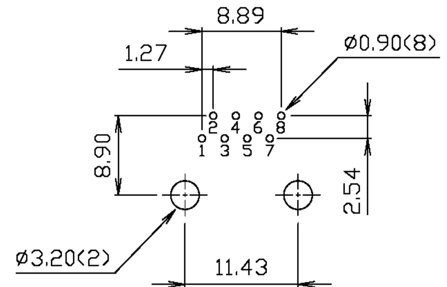
PC Board Layout Ref.
