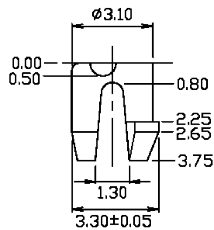
DETAIL X
