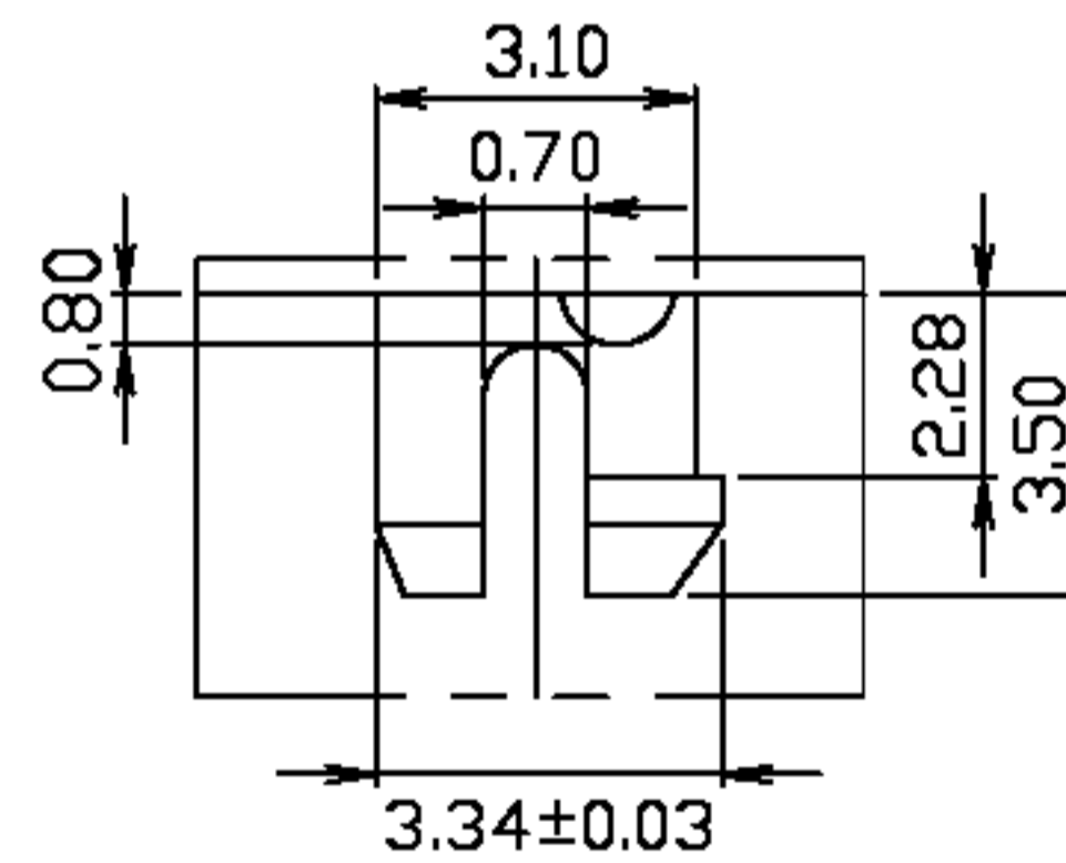
DETAIL X
