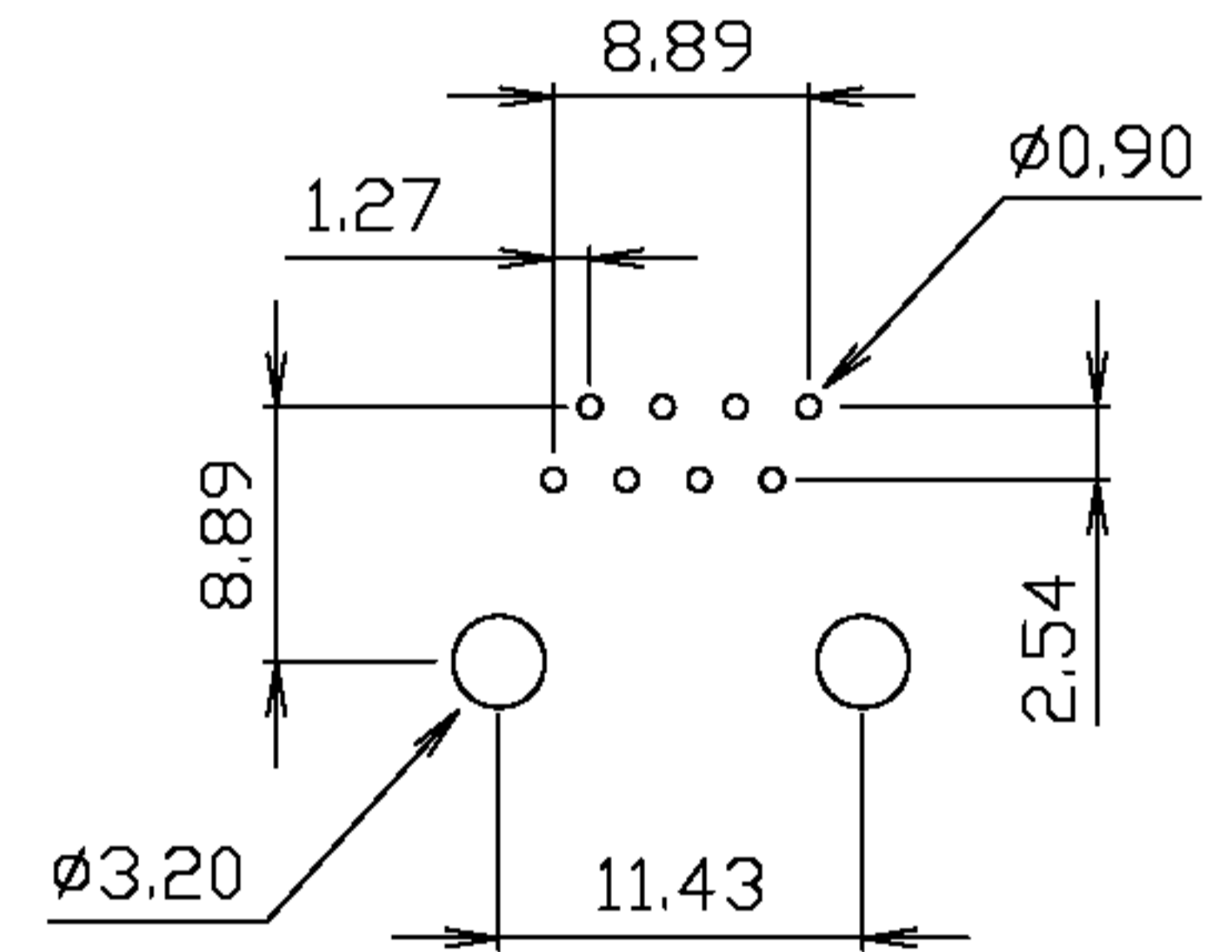
PC Board Layout
